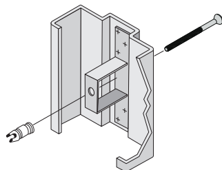
MASONRY WIRE ANCHOR
