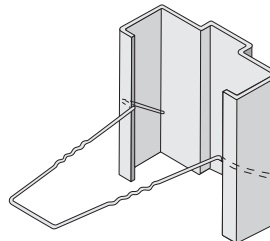
EXISTING OPENING ANCHOR (E.O.A.)
